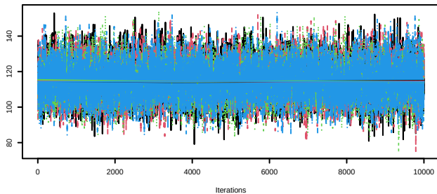
Trace of lambda.y.strd[1]
