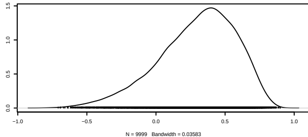
Density of lambda.y.strd[3]
