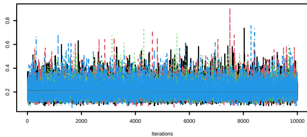
Trace of sigma.y[3]
