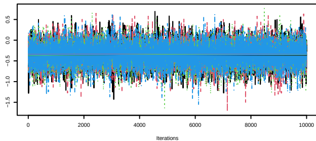
Trace of \nu.y[2]
