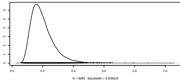
Density of \sigma.y[1]
